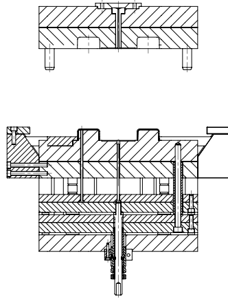
SECTION B-B EJECTOR PLATES BACK - MOLD OPEN
