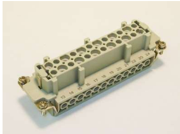
RPM0067 B24 Female Insert 16 amp TC12CxxG Thermocouple Cables
