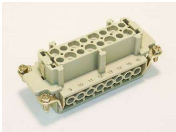
RPM0066 B16 Female Insert 16 amp TC8CxxG Thermocouple Cables
