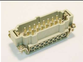
RPM0063 B16 Male Insert 16 amp MTC8G Mold Thermocouple Connector
